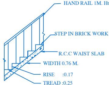
STAIR DETAIL
