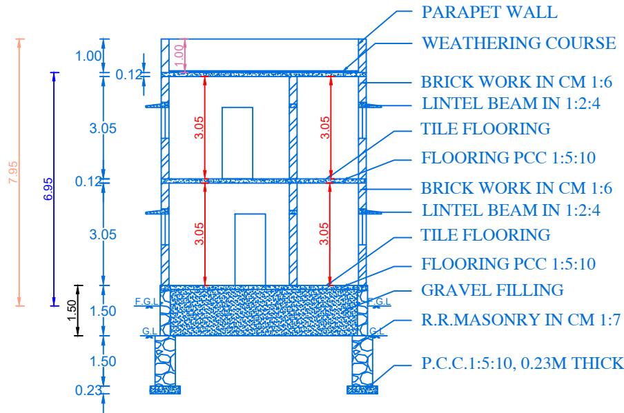
SECTION ON "V-B"
