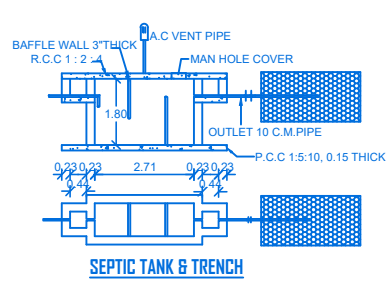
SEPTIC TANK & TRENCH
