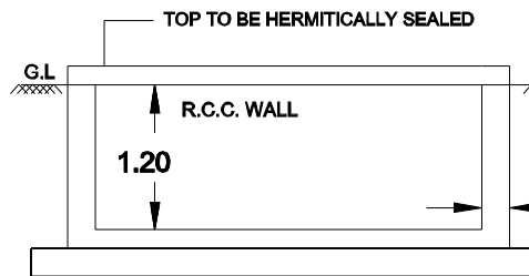
RWH SECTION
