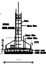
FOUNDATION DETAILS SCALE : 1:50.
