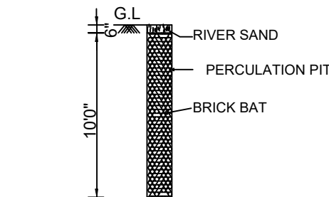
PERCOLATION PIT
