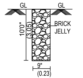
PERCOLATION PIT:-
