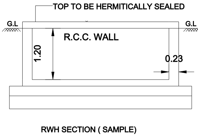
R.W.M. SECTION ( SAMPLE)
