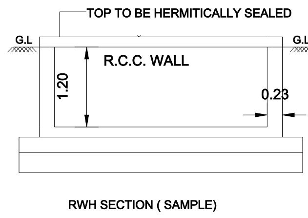
R/W SECTION ( SAMPLE)
