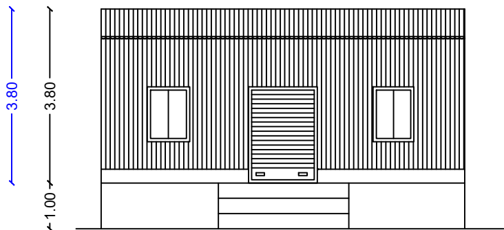
ELEVATION - EAST FACEING
