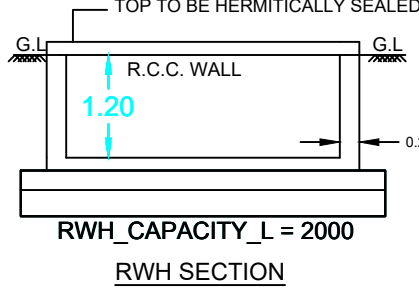
RWH SECTION
