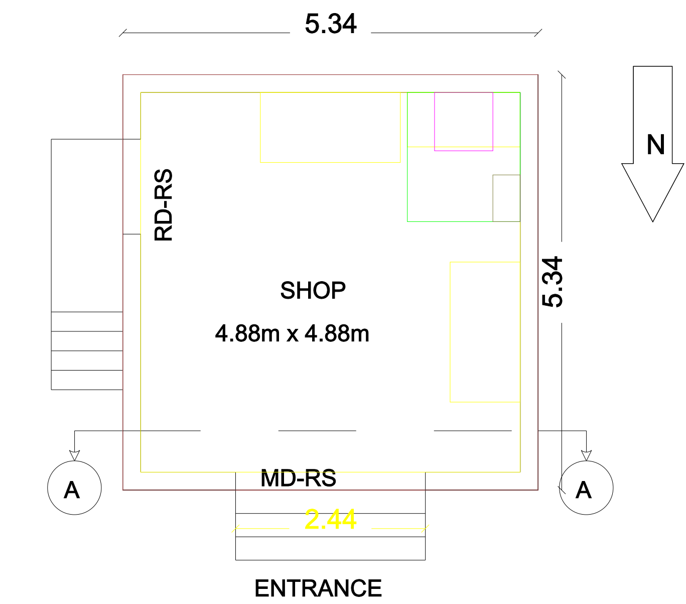
FLOOR PLAN
