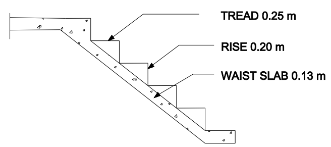
STAIR DETAILS
