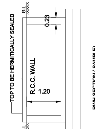
RCC WALL SECTION (SAMPLE)
