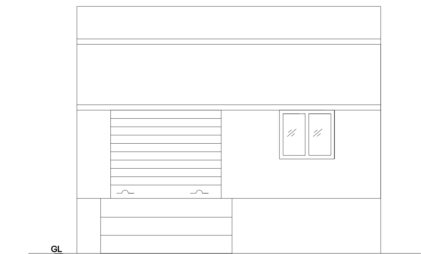
EASTERN SIDE ELEVATION
