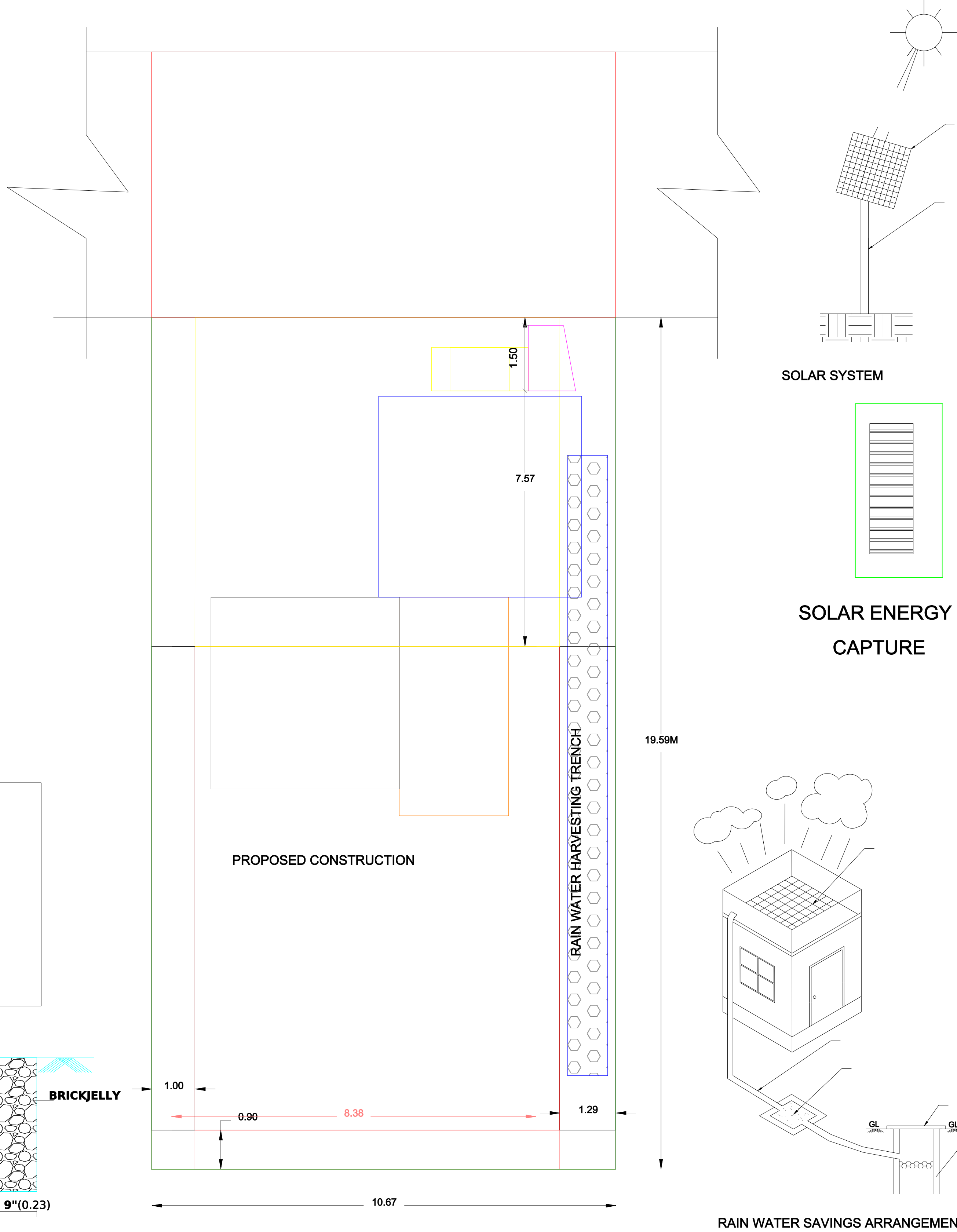
RAIN WATER SAVINGS ARRANGEMENTS
