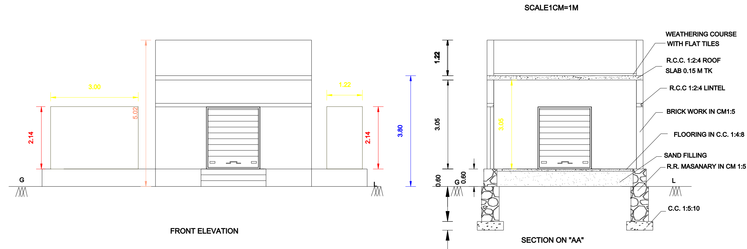
FRONT ELEVATION
