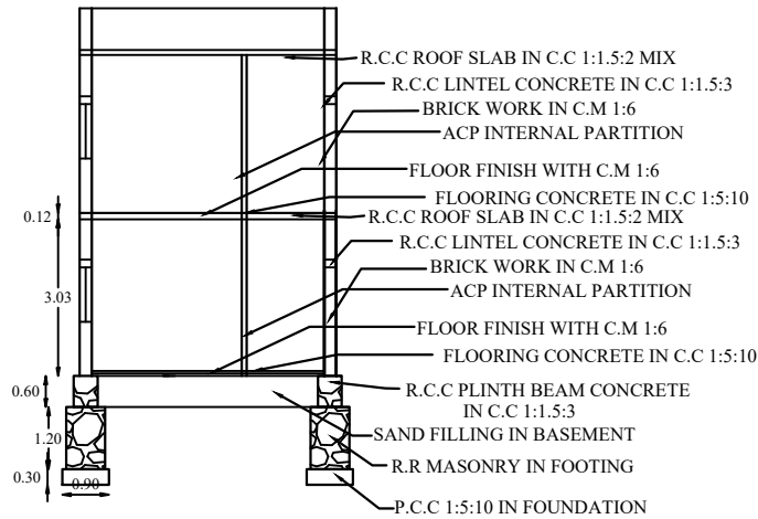
SECTION AB
