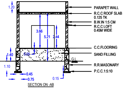
SECTION ON-AB
