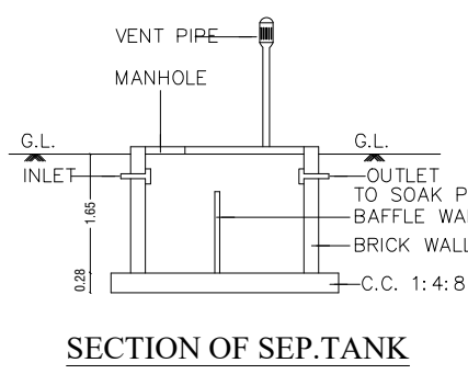
SECTION OF SEP.TANK
