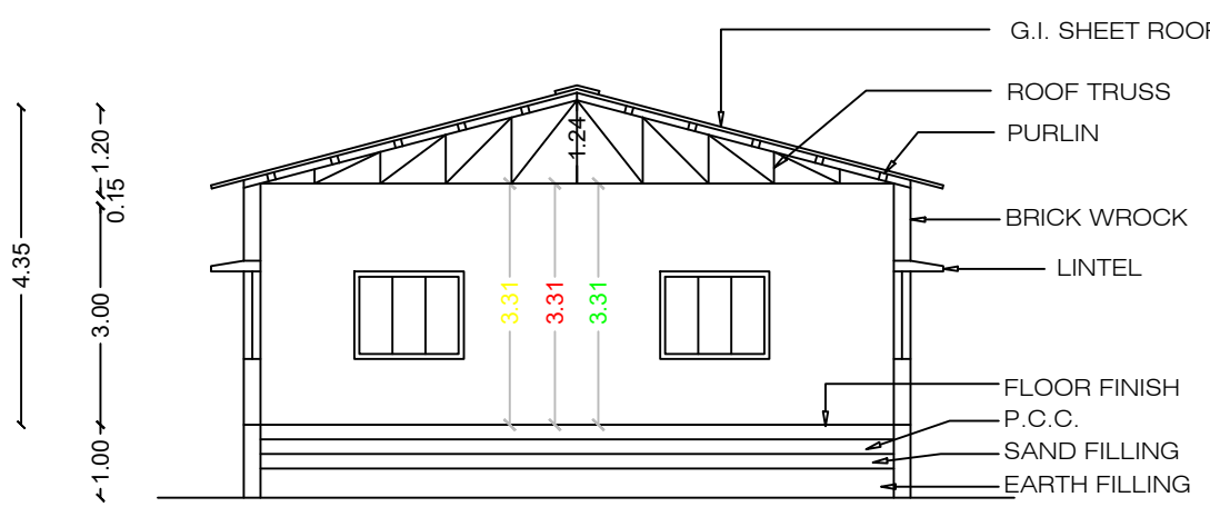
SECTION "XY"
