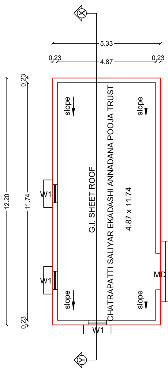
PROPOSED GROUND FLOOR PLAN ( G.I. SHEET ROOF )
