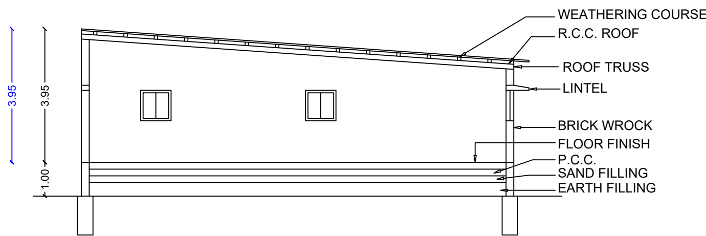
SECTION ON "XY"
