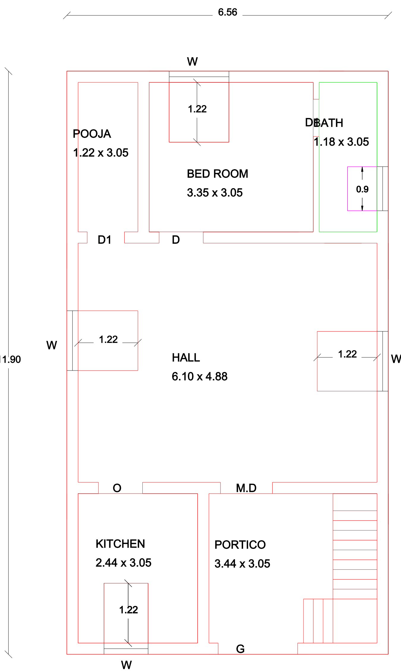
PLAN
