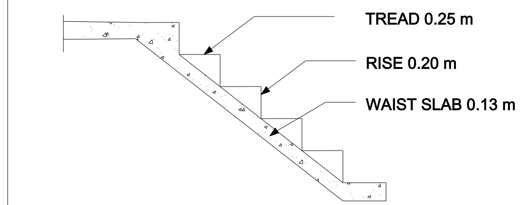
STAIR DETAILS
