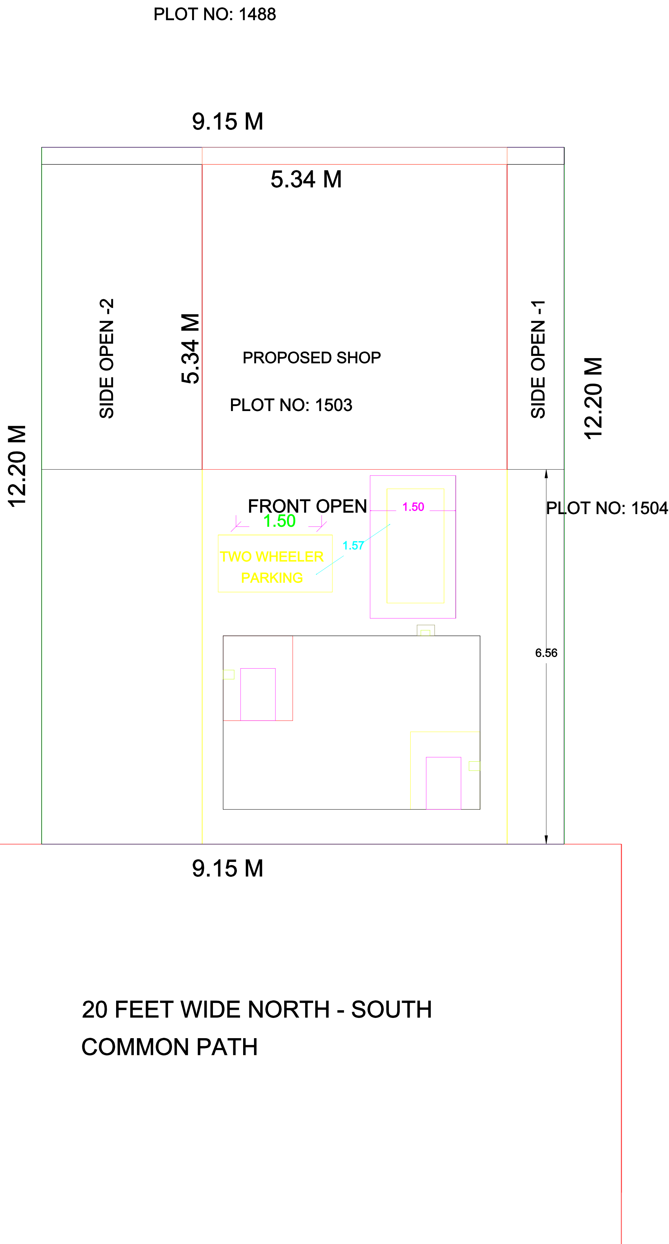
SITE PLAN
