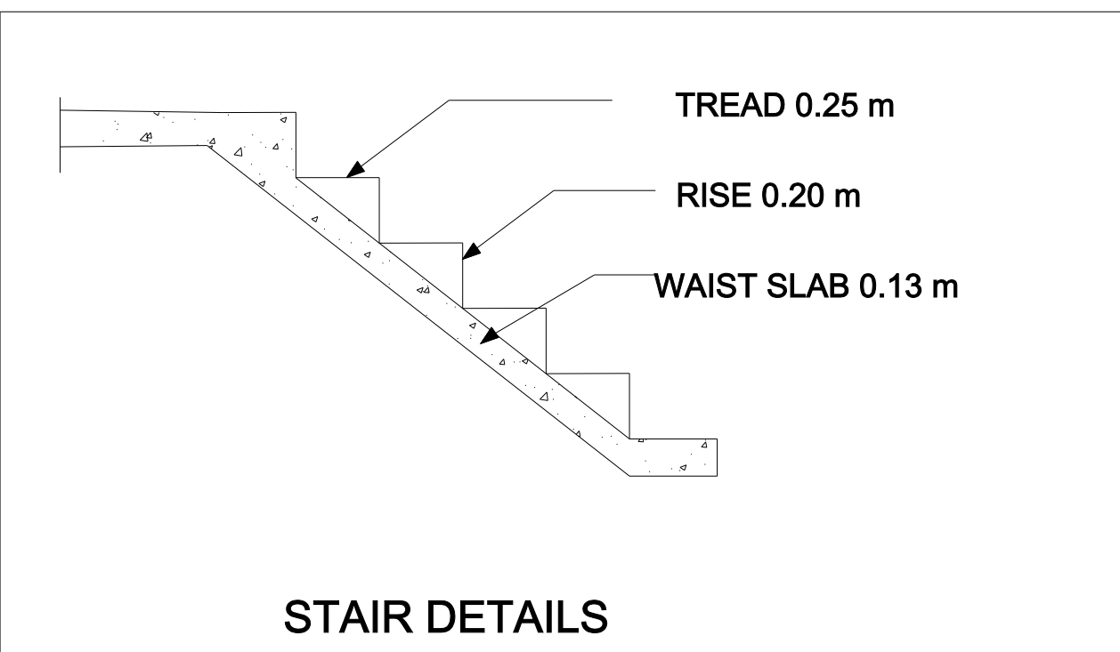
STAIR DETAILS
