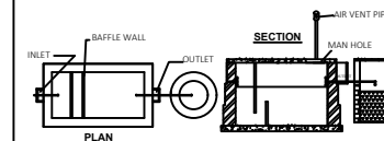
SEPTIC TANK DETAILS
