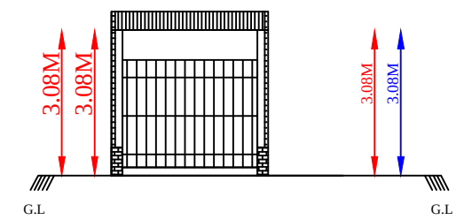
FRONT ELEVATION
