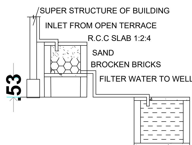
RAINWATER HARVESTING
