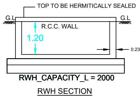
RWH SECTION
