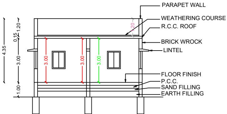
SECTION ON "XY"
