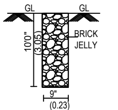
PERCOLATION PIT:-
