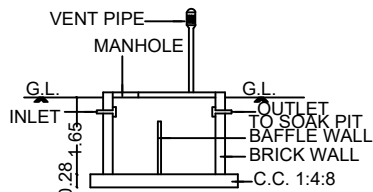
SECTION OF SEP.TANK
