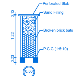
RAIN WATER COLLECTION WELL
