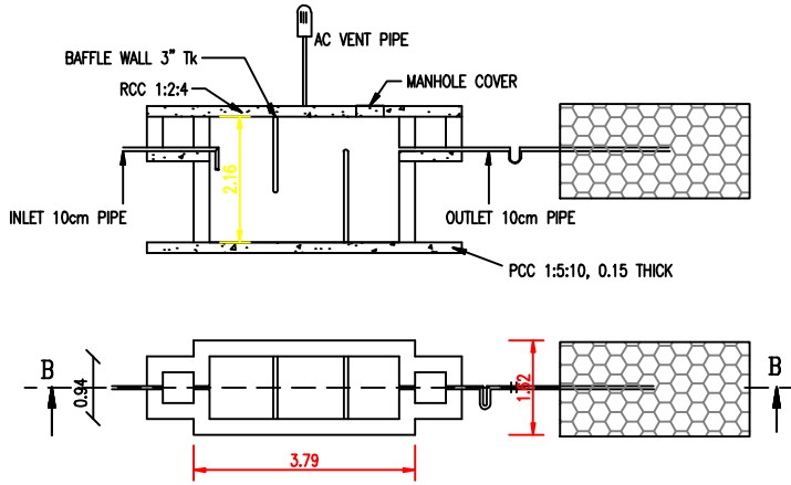
SEPTIC TANK AND TRENCH & U TRAP
