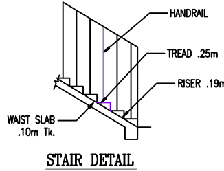
STAIR DETAIL
