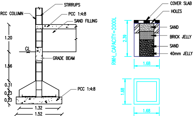
COLUMN DETAILS
