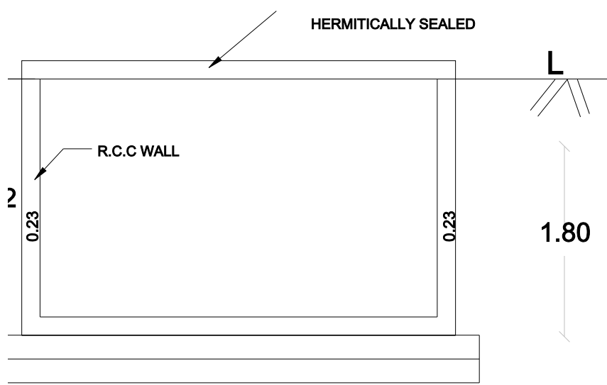
WATER HARVESTING
