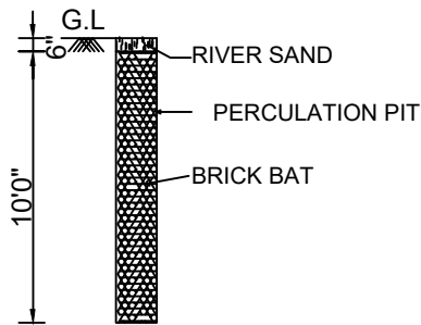
PERCOLATION PIT
