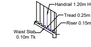
DETAILS OF STAIR CASE (SCALE 1:100)
