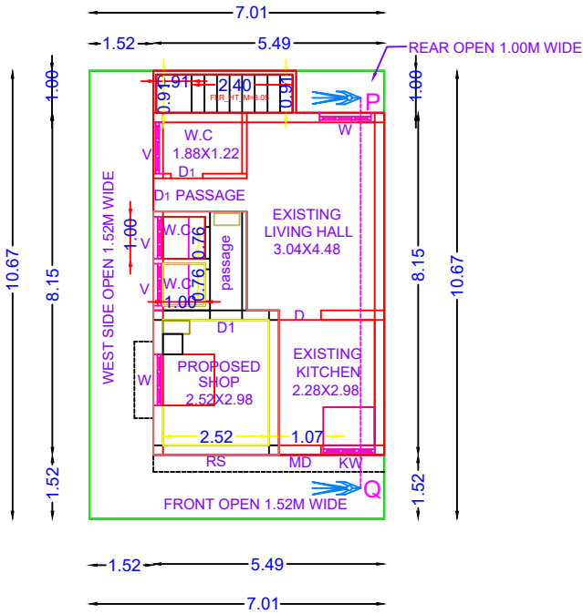
PARTLY EXISTING & PARTLY PROPOSED GROUND FLOOR PLAN
