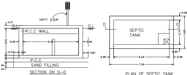
SCALE 1"=2'-0"
