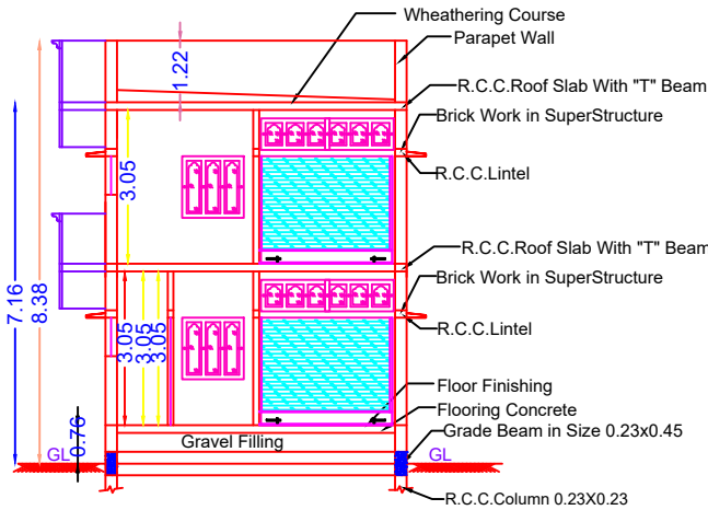
SECTION ON "PQ" SCALE 1:100
