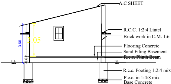
SECTION -"AB"
