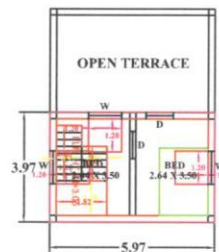
PLAN AT S.F.
