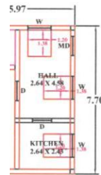
PLAN AT F.F.
