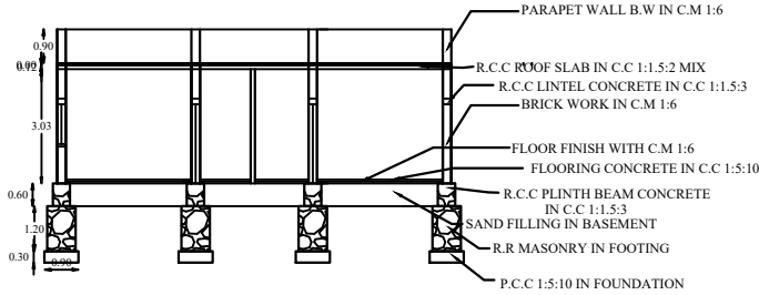
SECTION AB
