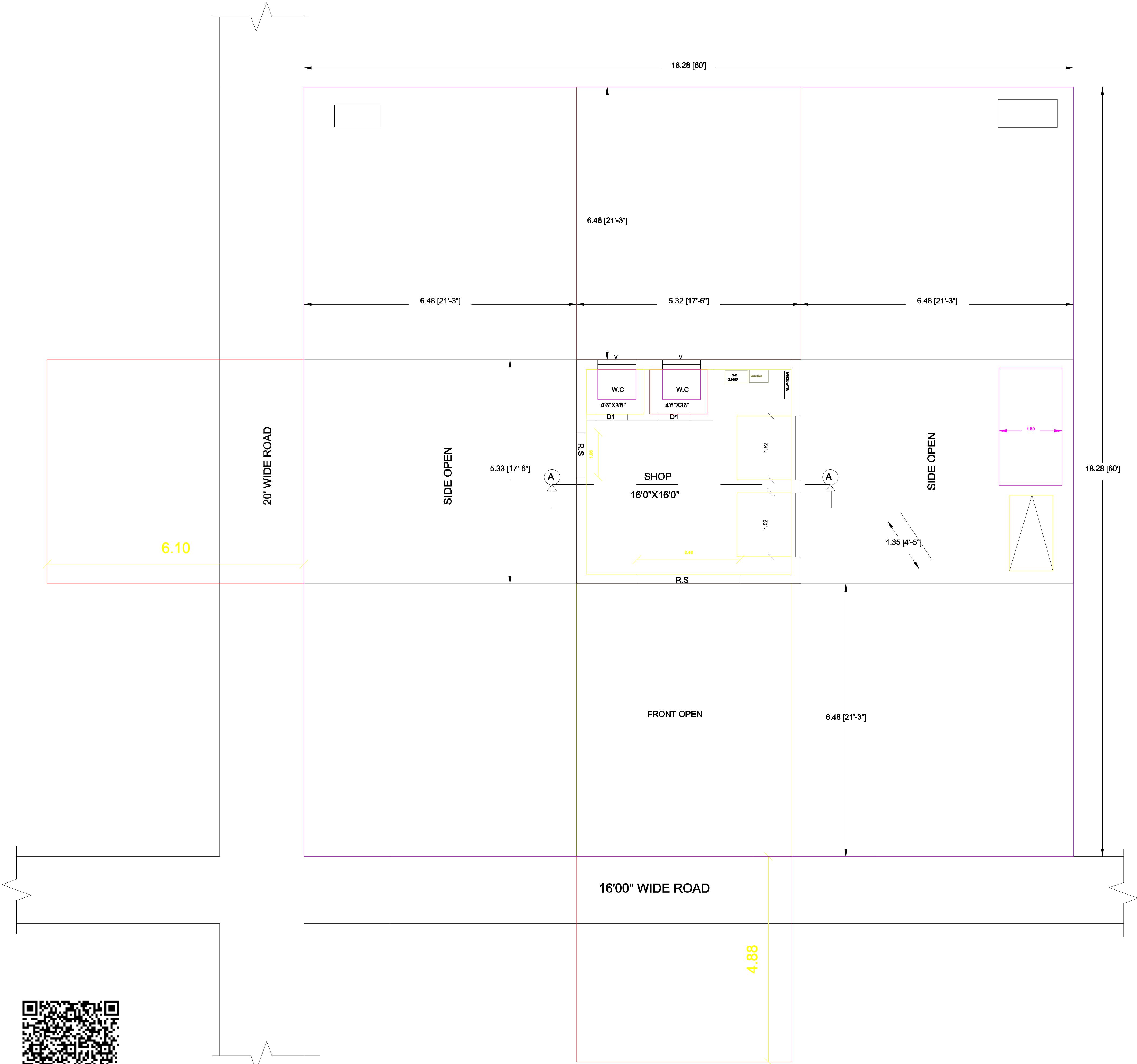
PRO.GROUND FLOOR PLAN
