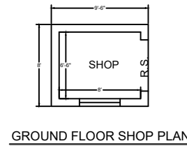
GROUND FLOOR SHOP PLAN
