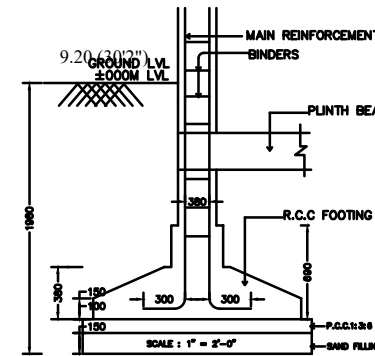
TYPICAL SECTION OF R.C.C COLUMN FOUNDATION
