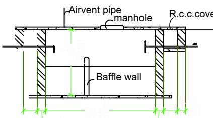
SEPTIC TANK DETAILS (NTS)
