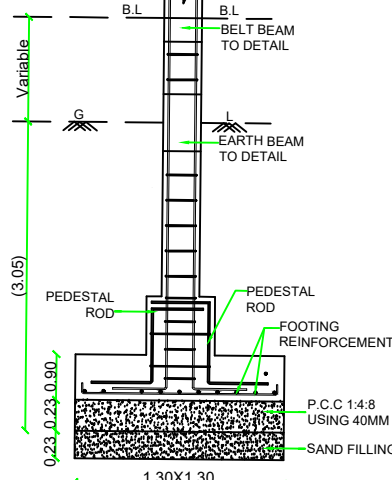
FOUNDATION DETAILS DETAILS-AA
