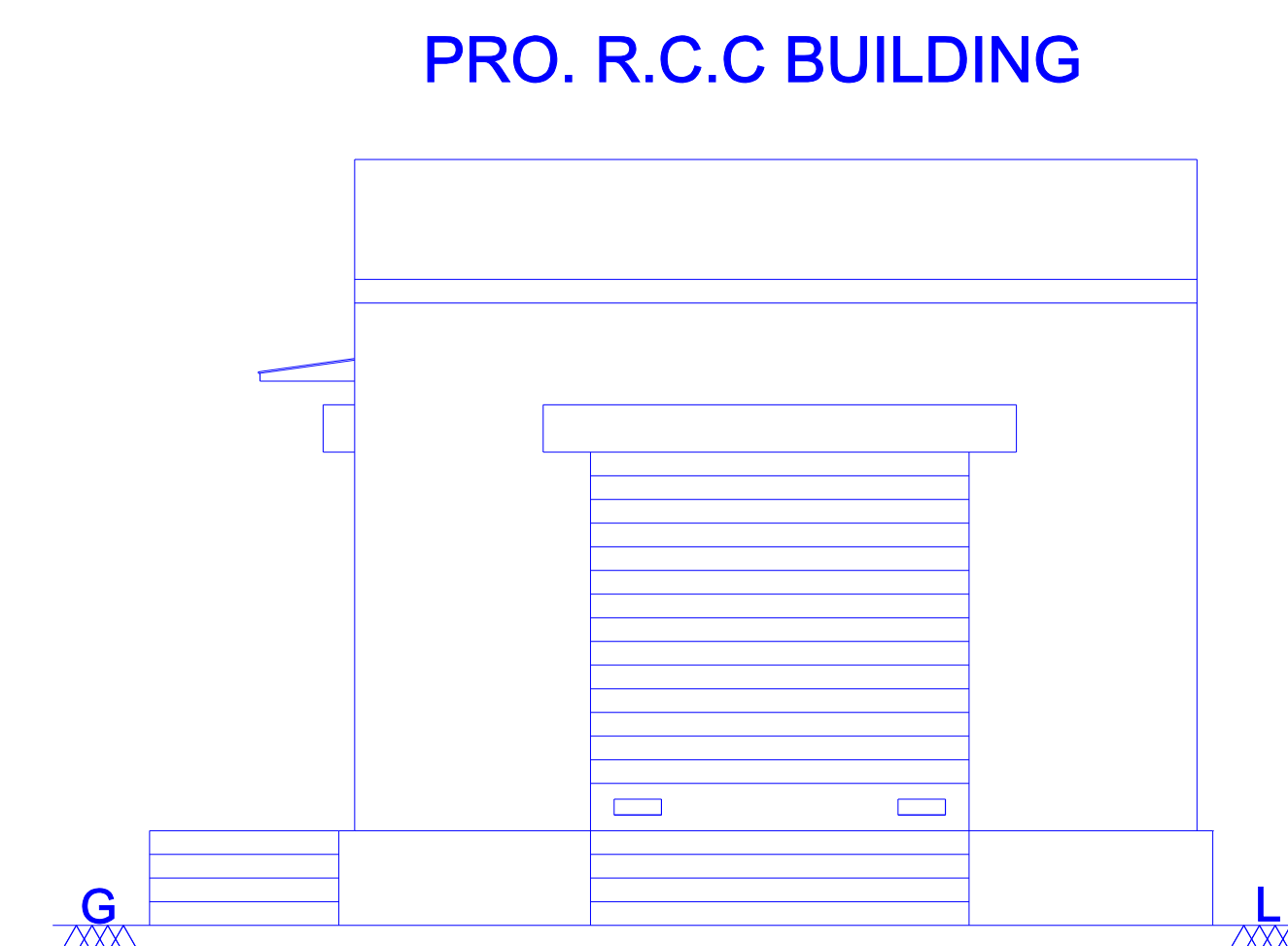
ELEVATION ON NORTH SIDE
