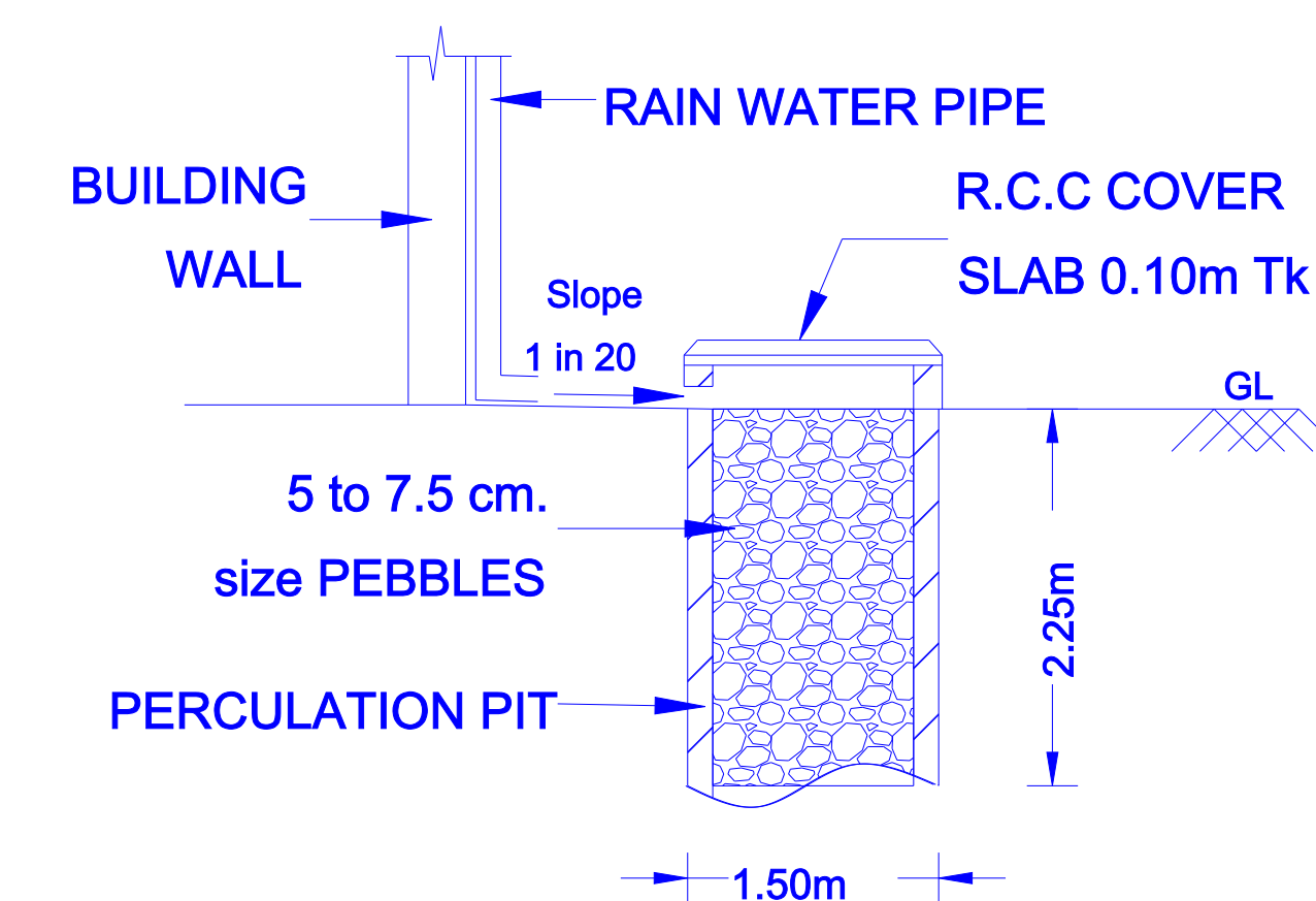
RAIN WATER HARVESTING TRENCH PIT DETAILS
