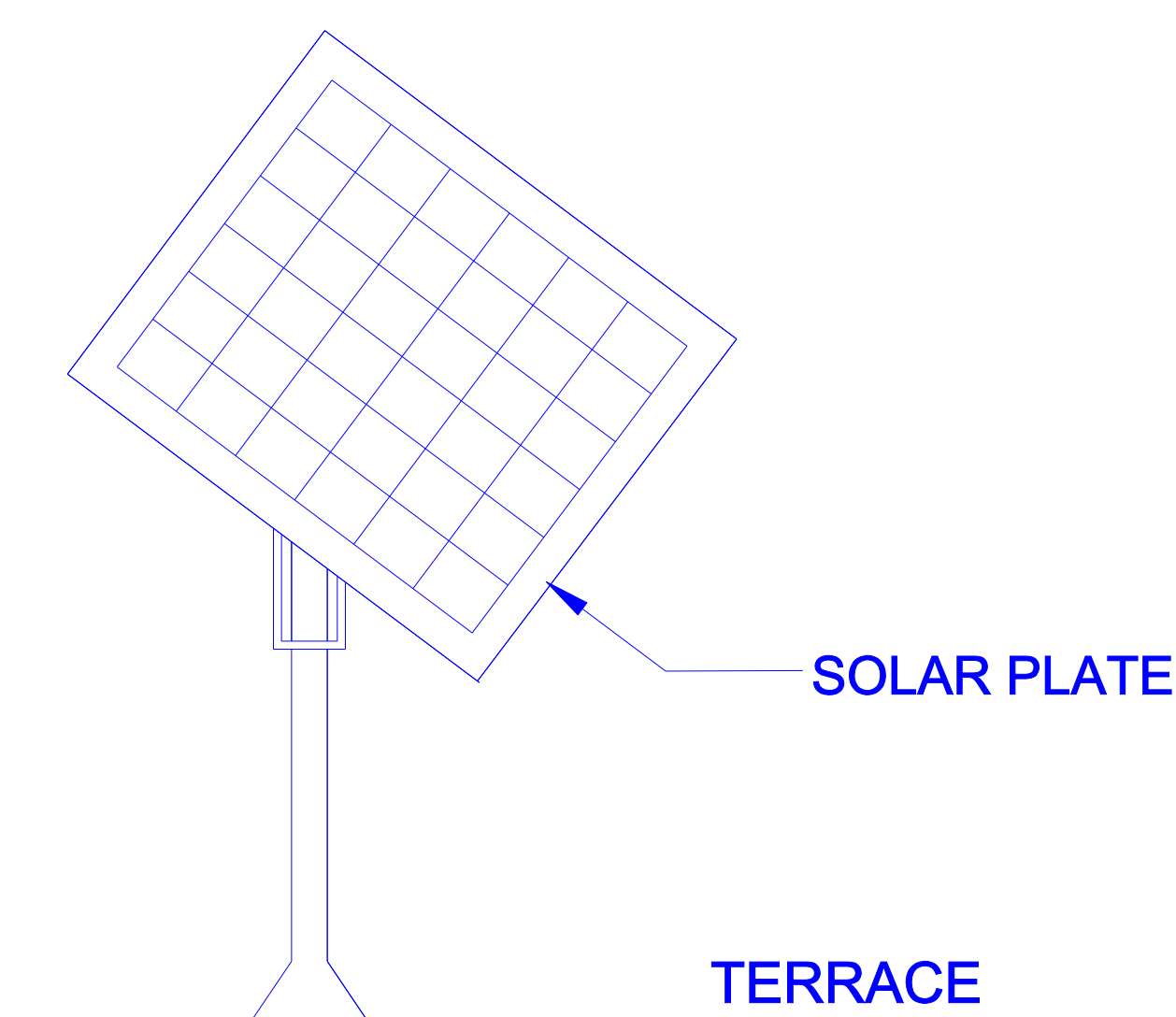
SOLAR SYSTEM
