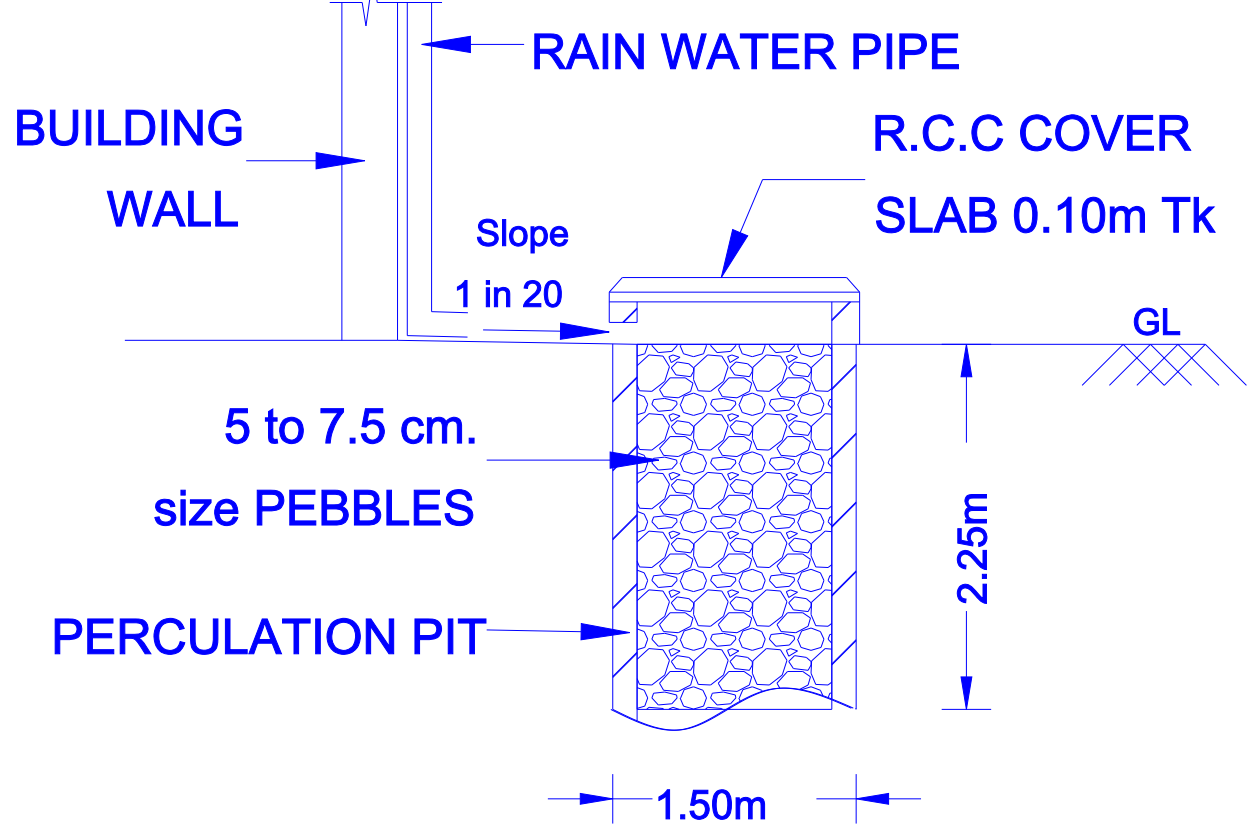
RAIN WATER HARVESTING TRENCH PIT DETAILS
