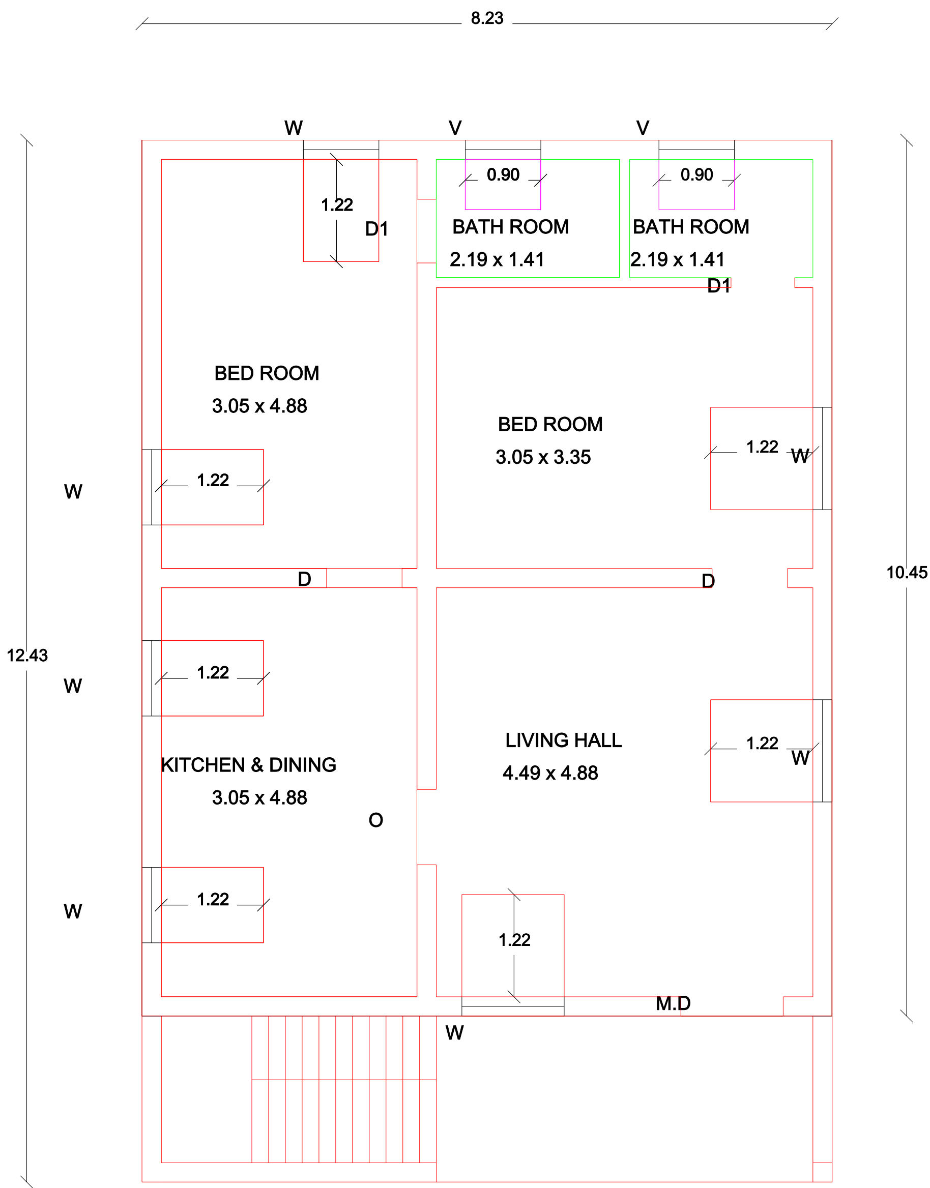
PLAN
