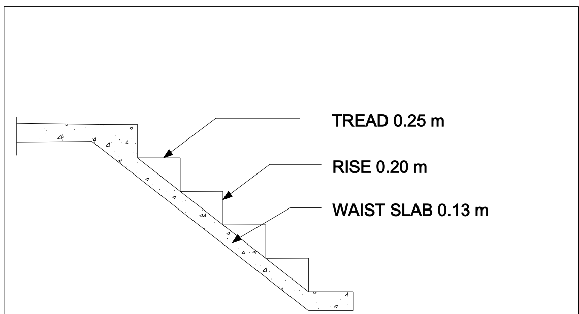
STAIR DETAILS
