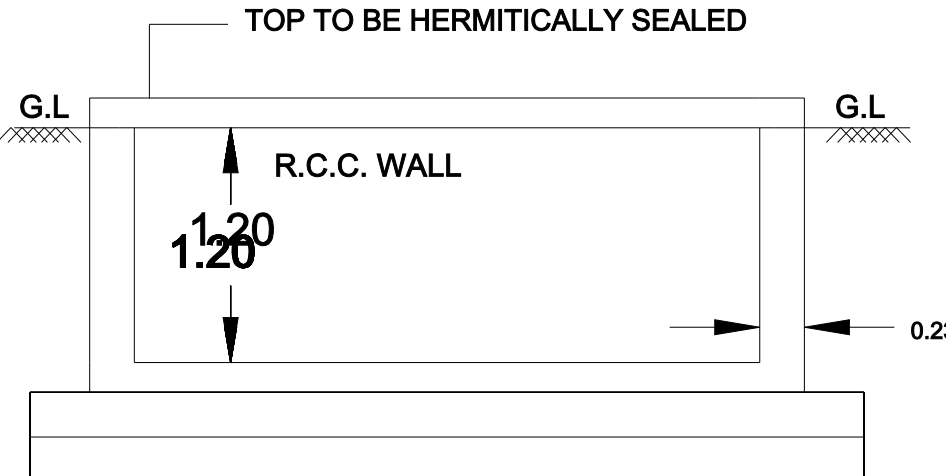
RW SECTION
