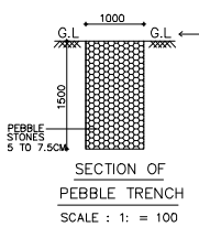
SECTION OF PEBBLE TRENCH SCALE : 1" = 10'
