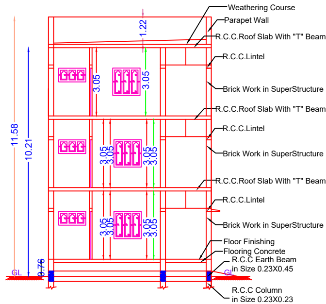
SECTION ON "PQ"
