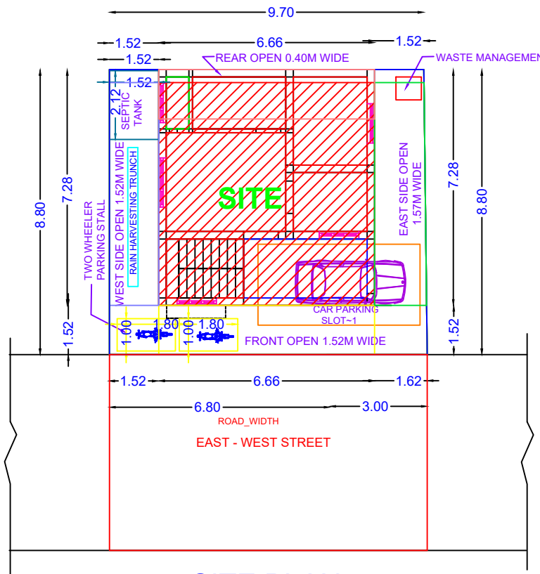
SITE PLAN
