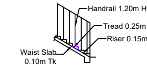
DETAILS OF STAIR CASE
