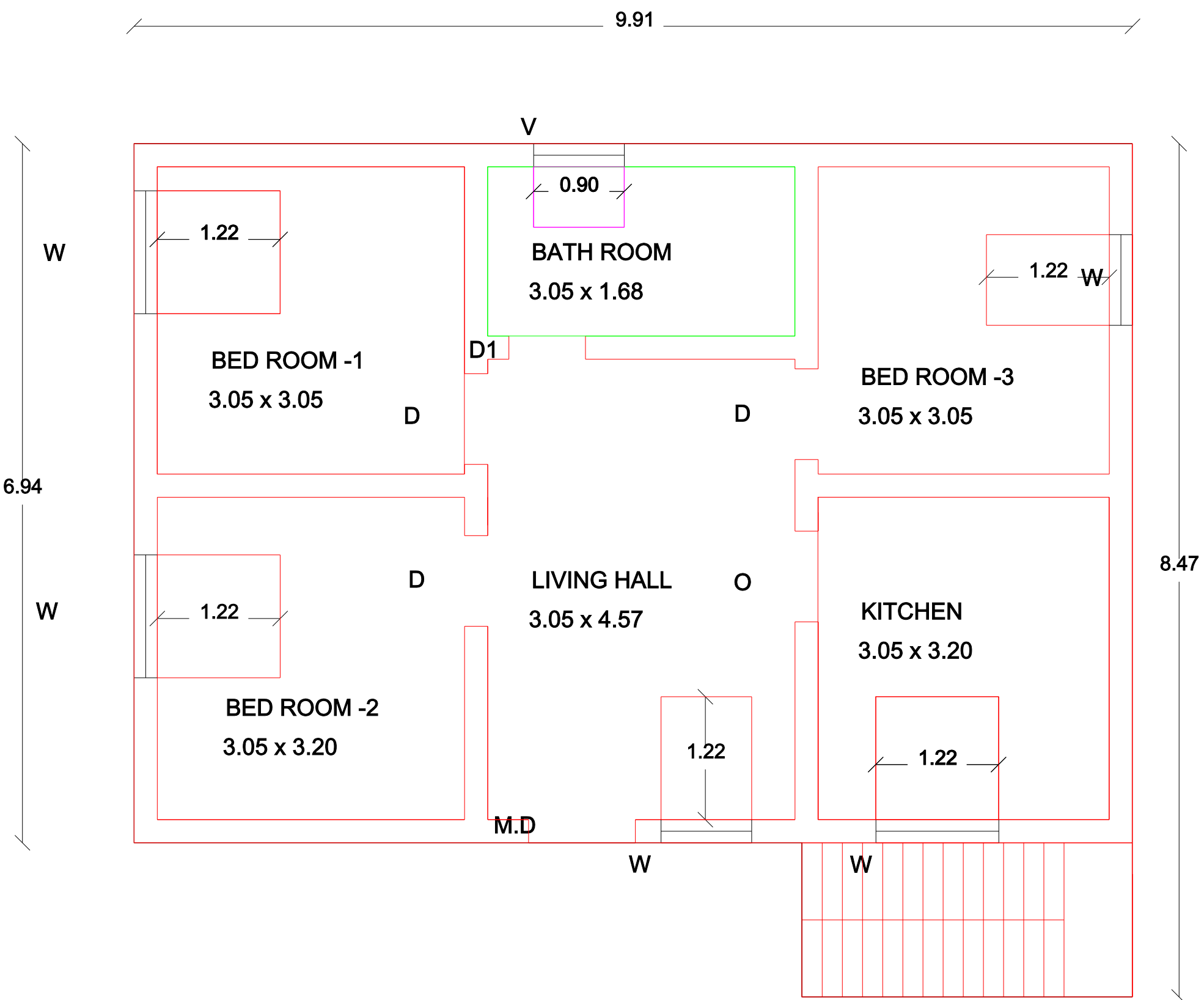
PLAN
