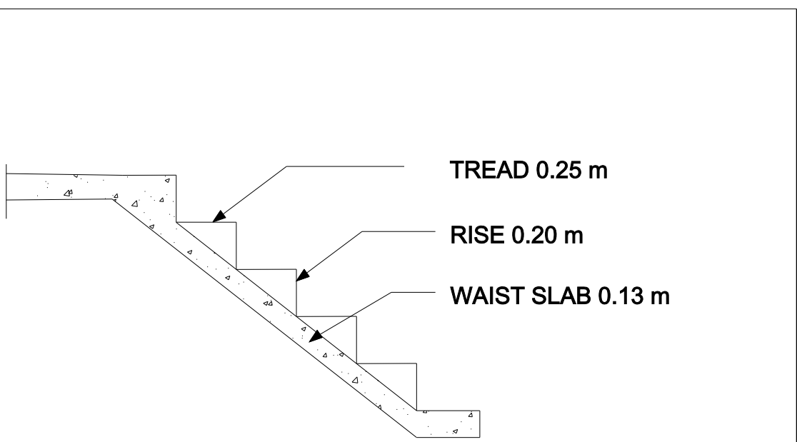
STAIR DETAILS
