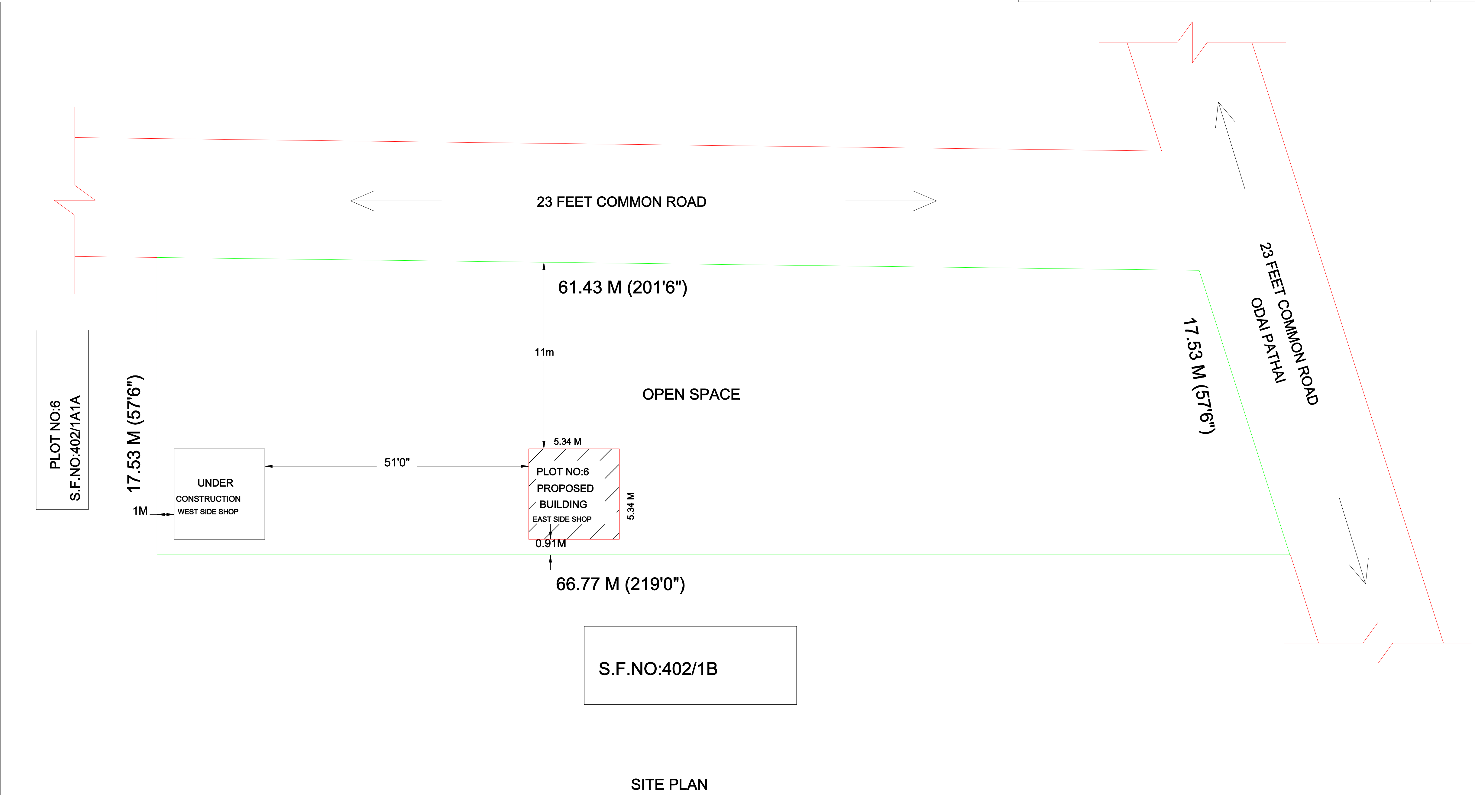
SITE PLAN
