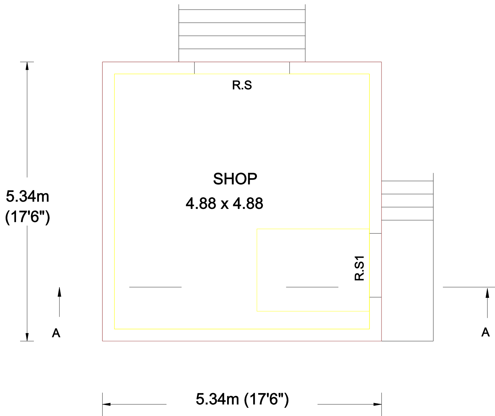
BUILDING PLAN
