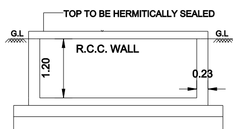
RAIN SECTION (SAMPLE)
