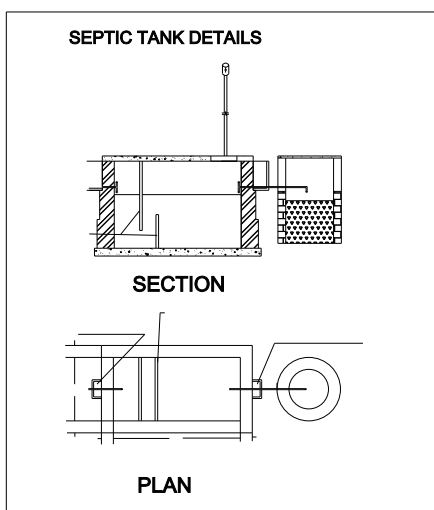
SECTION
