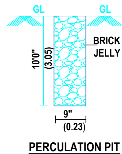
PERCOLATION PIT
