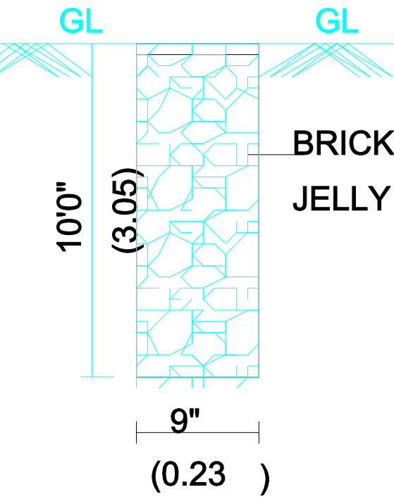
PERCULATION PIT
